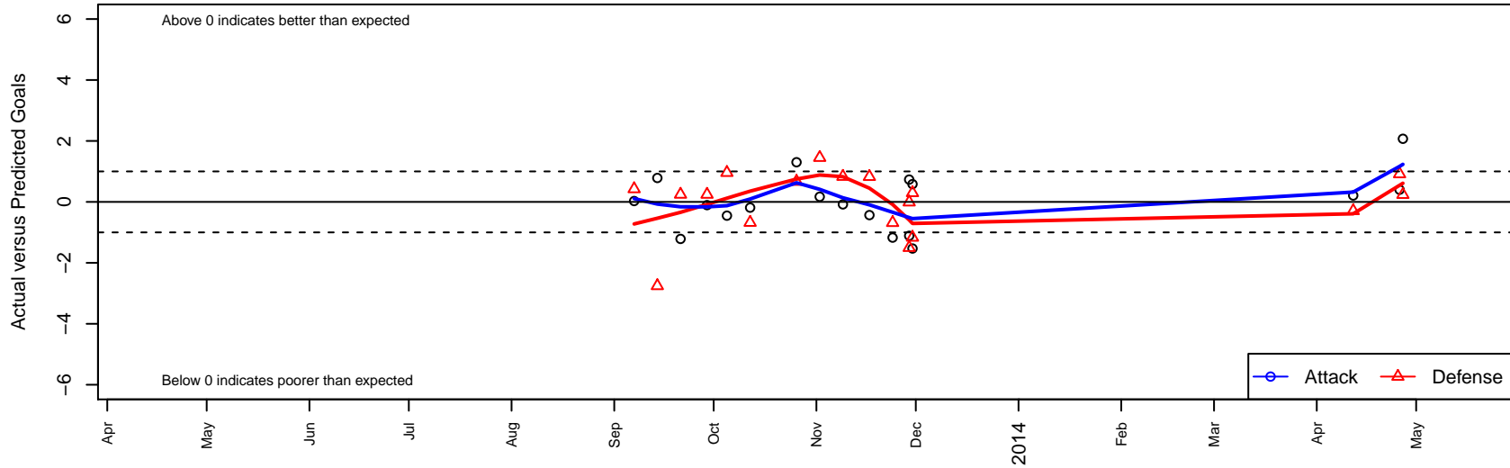
Encinitas Express White B99 Dots are actual minus expected GF (blue circles) and GA (red triangles). Blue line is smoothed change in attack strength. Red is smoothed change in defense strength.
